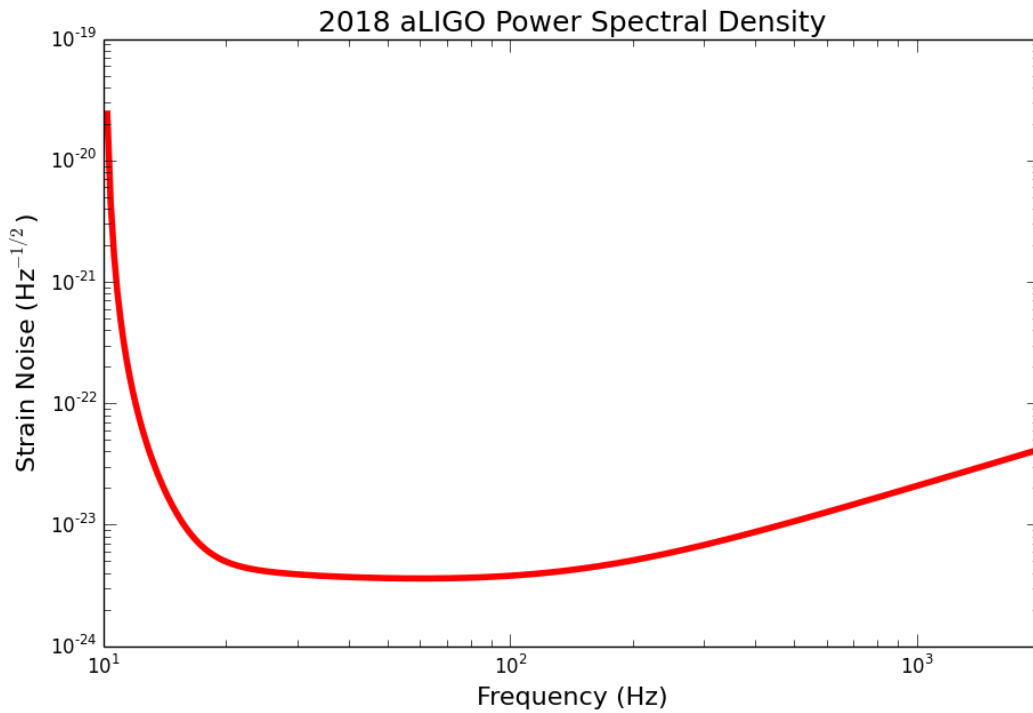
Figure 30: Simulated 2018 aLIGO power spectral density used in the ETG mock data challenge. The simulated PSD provides the noise power spectrum for aLIGO under the high-power broad-band signal recycling (no detuning of the signal recycling cavity), and includes thermal and quantum noise.
