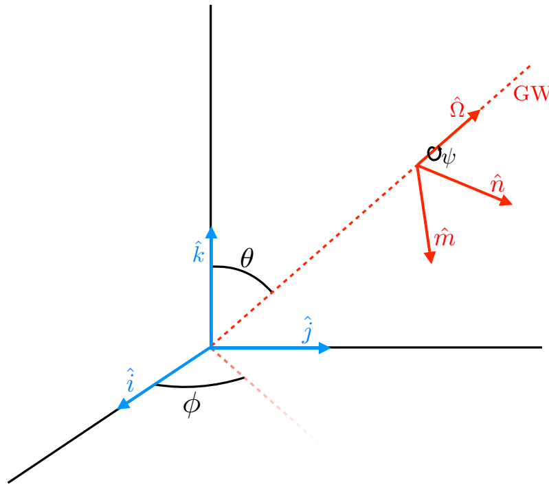
Figure 2: Illustration of a possible gravitational-wave coordinate system. The wave propagates in the direction \hat{\Omega} , and the vectors m and n , obtained through rotations of the angle \psi , represent the most general choice of coordinates.
